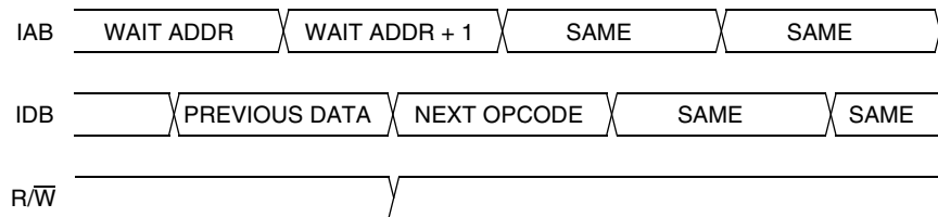
Figure 5-15. Wait Mode Entry Timing
